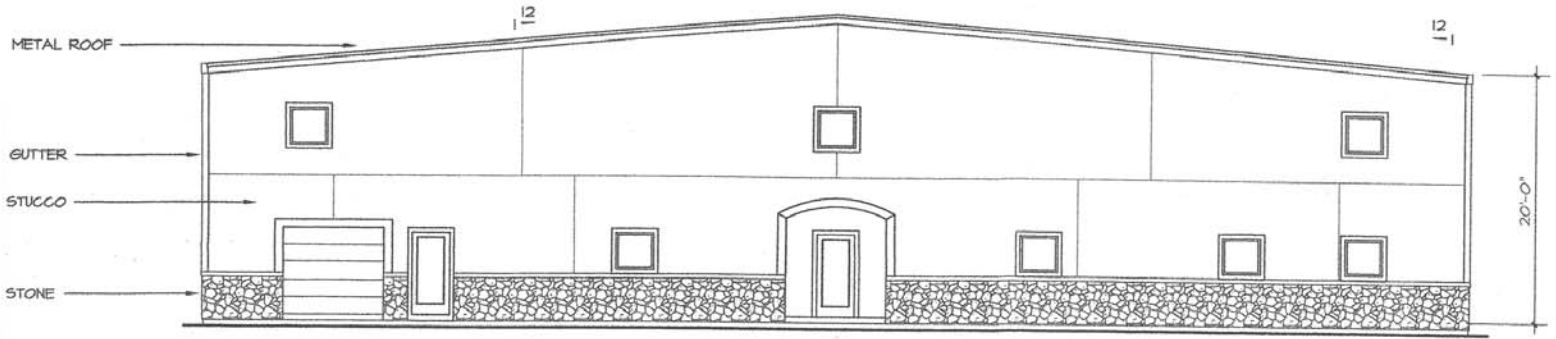
front elevation
